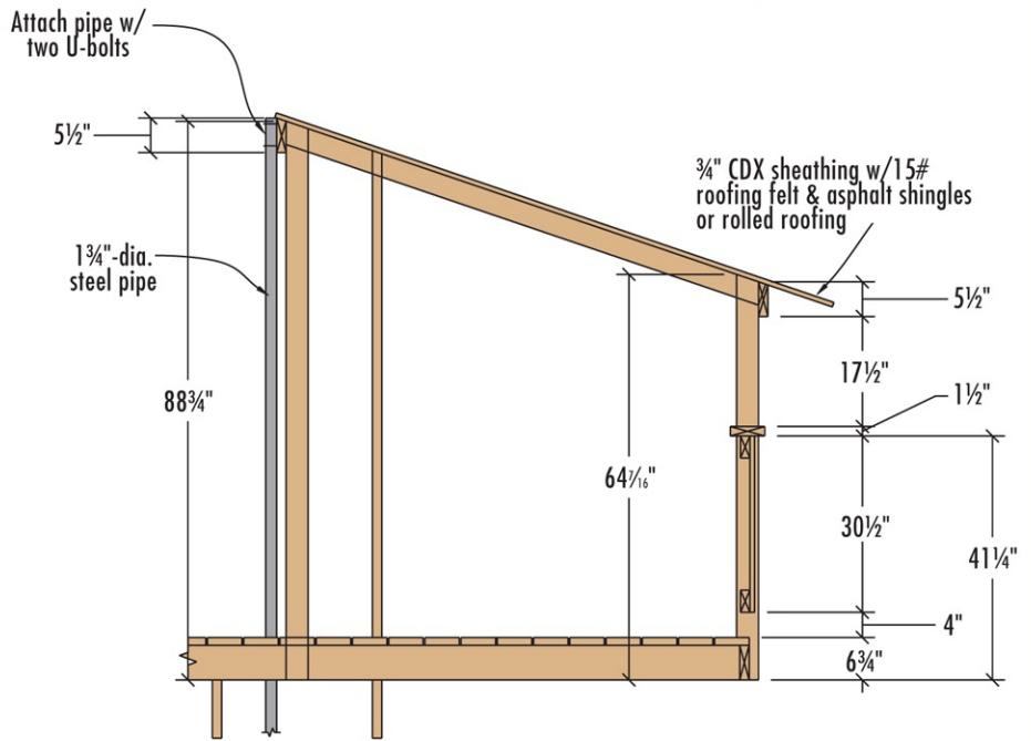
SIDE SECTION @ ROOF/RAILING
