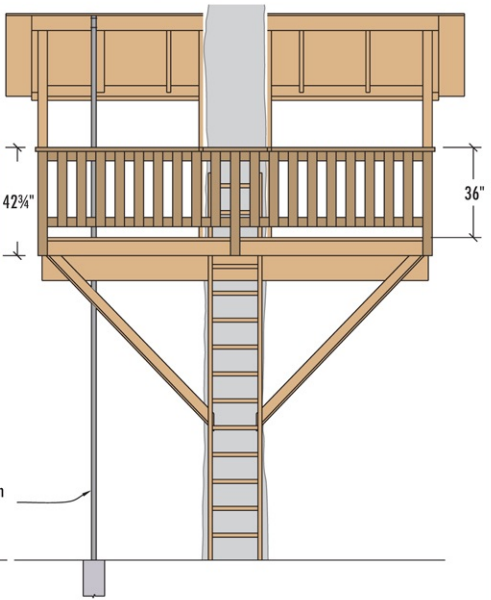
ELEVATION & LADDER
