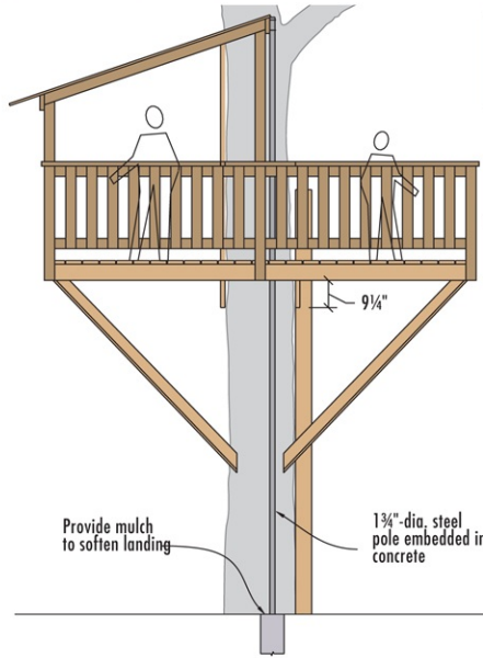
ELEVATION & SIDE
