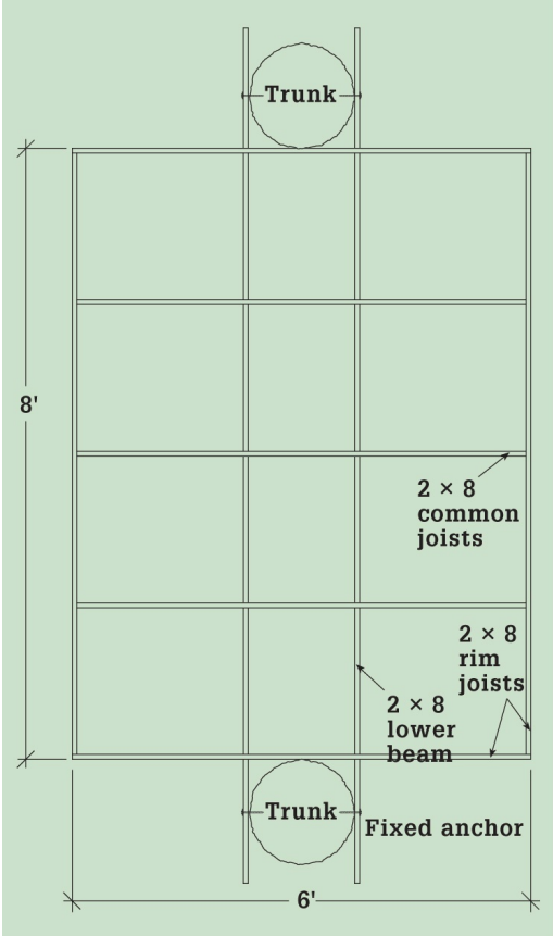
Two-trunk treehouse platforms require more planning and engineering but can support a larger structure.
