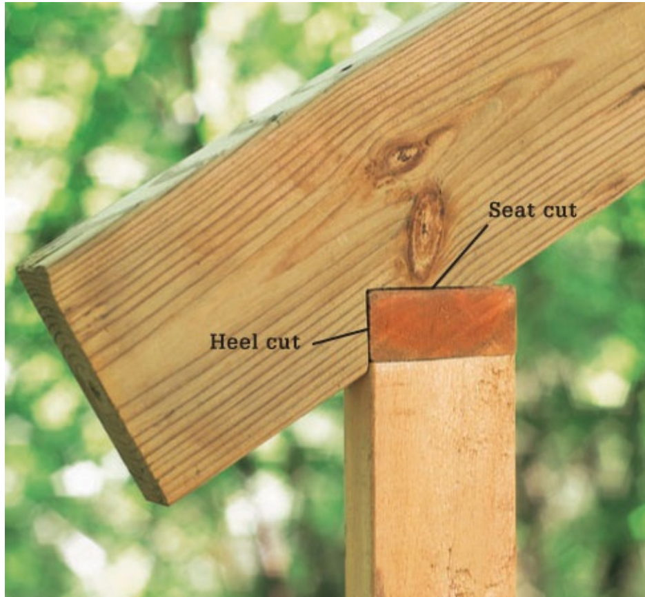
The angles of a bird's mouth cut for a 30° roof pitch.
