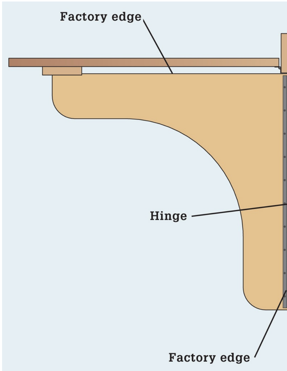
The swing-out brace has symmetrical curves cut into its front edge and uses the plywood's factory edges for its top and rear finished edges.
