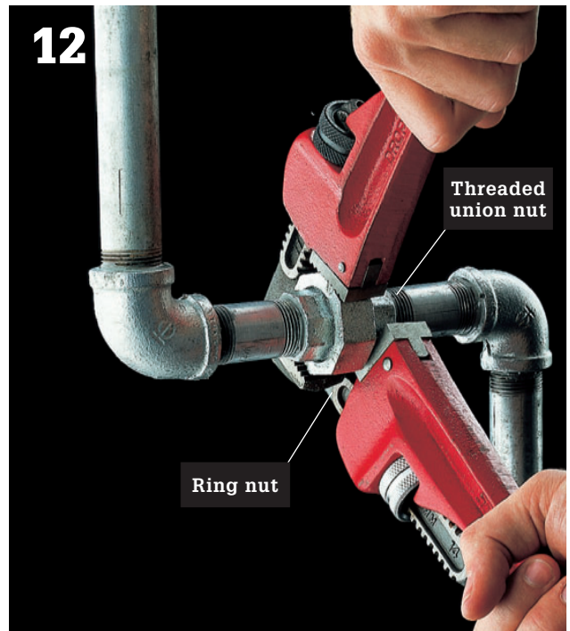
Complete the connection by screwing the ring nut onto the threaded union nut. Tighten the ring nut with pipe wrenches.
