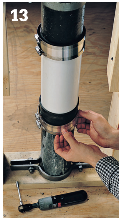
13 Slide stainless steel bands and clamps over the neoprene sleeves.
