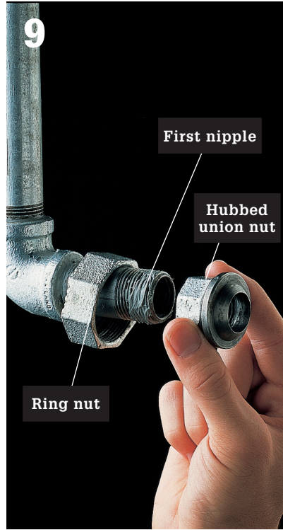
Slide a ring nut onto the installed nipple, then screw the hubbed union nut onto the nipple and tighten with a pipe wrench.
