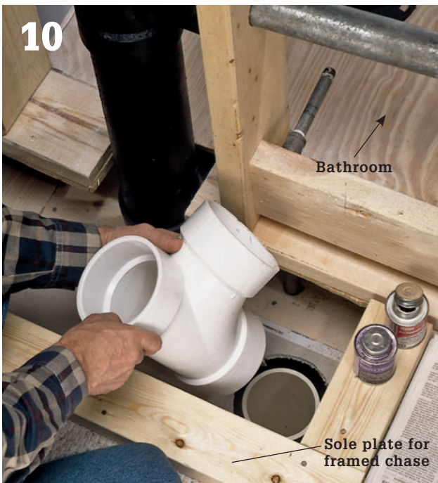
10 Attach the next waste T-fitting to the stack. In our demonstration project, the waste-T lay between floor joists and was used to connect the toilet drain. Make sure the waste-T is positioned at a height that will allow for the correct \frac{1}{4} " per ft. downward slope for the toilet drain.
