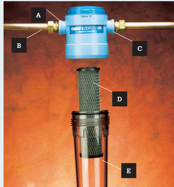
A whole-house water filtration system: (A) intake side, (B) supply pipe from the water meter pipe, (C) outtake side to the house supply pipe, (D) filter, and (E) filtration unit cover.
