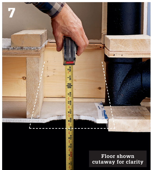
Determine the length for the next piece of waste-vent pipe by measuring from the basement T-fitting to the next planned fitting in the vertical run. In our project, we installed a T-fitting between floor joists, where the toilet drain was connected.
