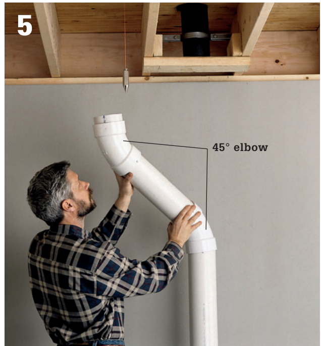
Dry-fit 45° elbows and straight lengths of plastic pipe to offset the new stack, lining it up with the plumb bob centered on the ceiling opening.
