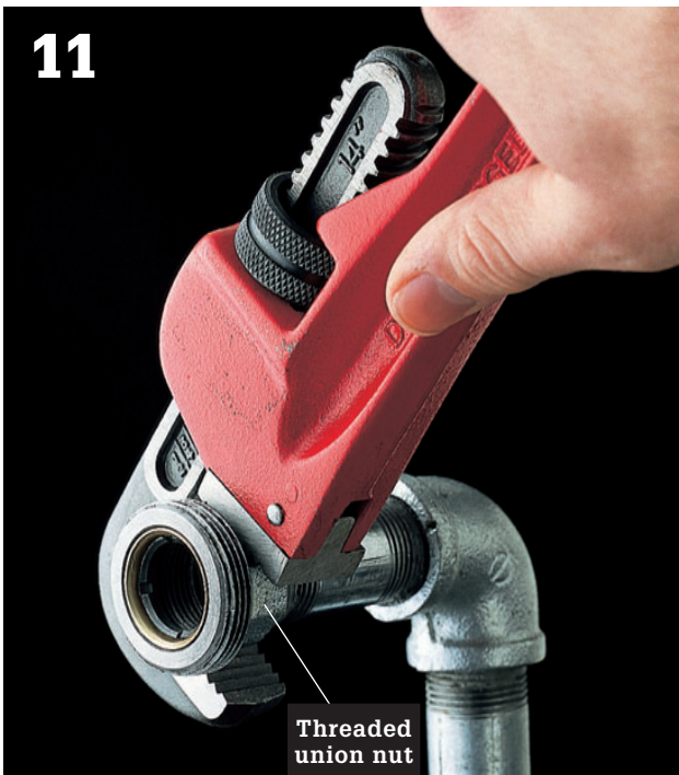
Screw the threaded union nut onto the second nipple. Tighten with a pipe wrench. Turn pipes into alignment, so that the lip of the hubbed union nut fits inside the threaded union nut.
