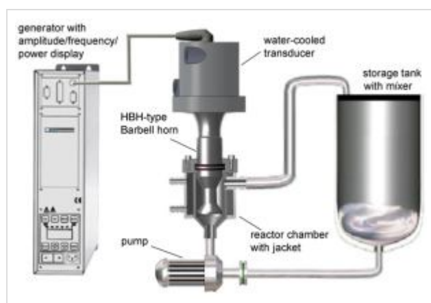
Picture: Schematic of bench and industrial-scale ultrasonic liquid processors showing the liquefaction principle.
