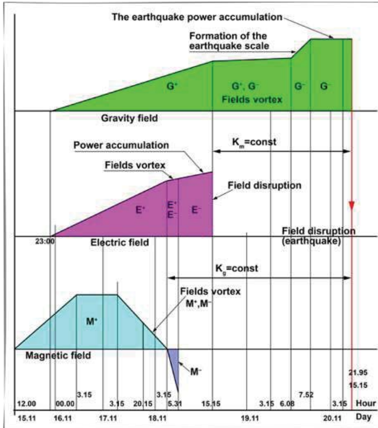
The conventional graph of the above tables on the earthquake
