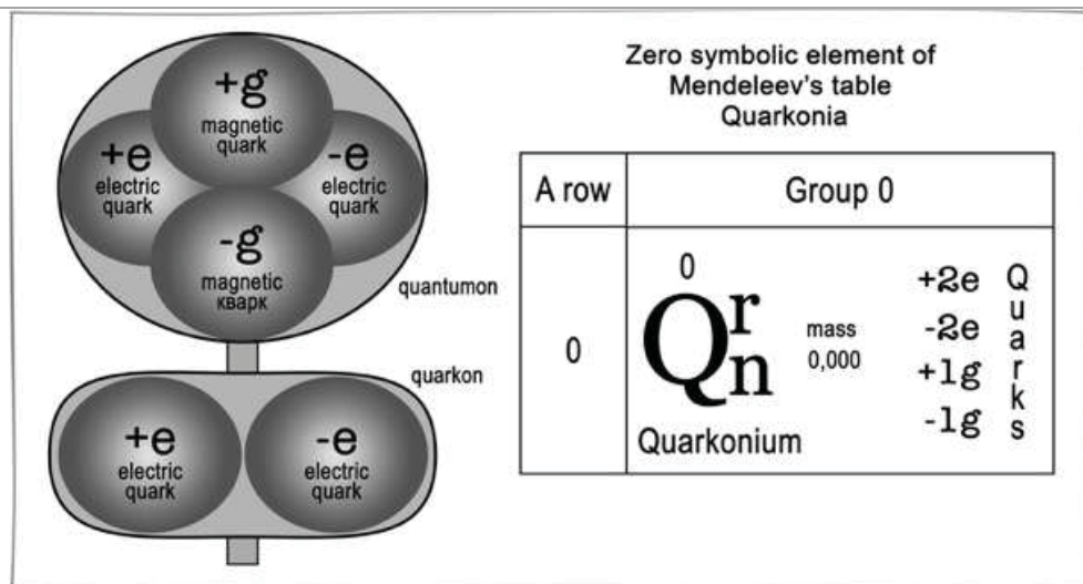
Graphical presentation of the symbolic zero element of Mendeleev's table Quarkonia in the form of an energy cross of quarks in the composition of the quantum
