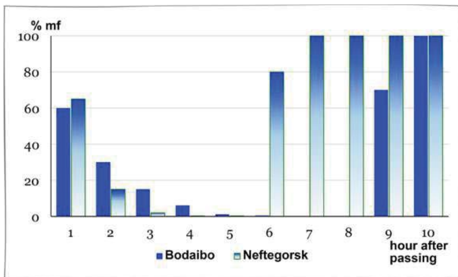
The time after which an earthquake occurs (after 100% field passing) in cities
