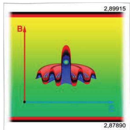
Electrical (E) and magnetic (B) fields astha aconsequence of dimensionality differential
