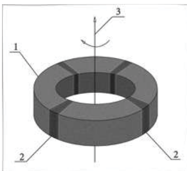
The generator of the axion field: 1 – Ferromagnetic material, 2 – Permanent magnets, 3 – The rotation size is: 020×012, height – 6 mm.
