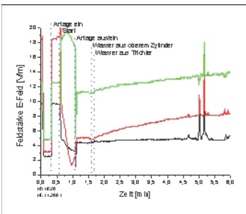
Figure23: all devices on, EMF antenna mounted
