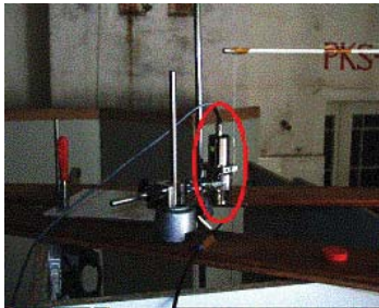
Figure 11: Probe for measuring the electrostatic field
