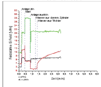
Figure28: EMS-100 filter setting to 50 Hz
