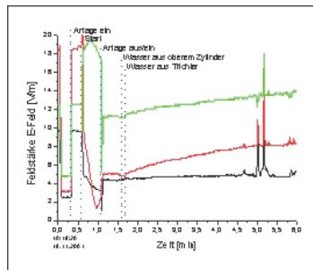
Figure24: all devices on, EMF antenna removed
