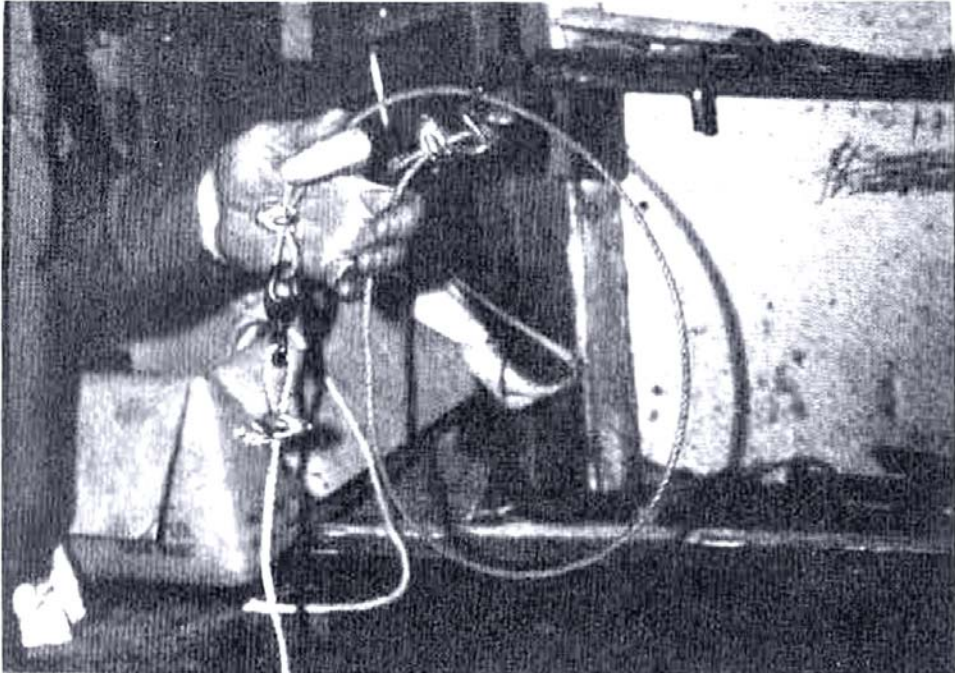
A trapper's bear snare made from steel cable, cable clamps, T lock, and a swivel. Ideally, the T lock shown should face the opposite direction.
