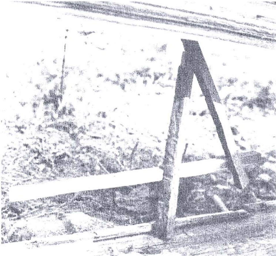
Top: Three sticks needed for figure-four trigger. Note that the longest piece has two notches cut into it. Bottom: Deadfall with figure-four trigger in place. Bait is wired to the long horizontal piece, which also contains the two notches.
