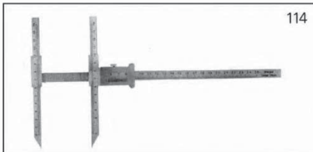
Calipers for measuring the absolute and projected dimensions of the face. Length: 0-250 mm/0-140 mm. Weight: 0.300 kg.
