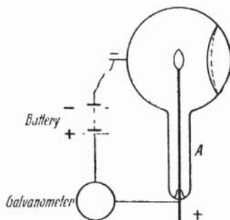
Figure 19. Photoelectric cell.
