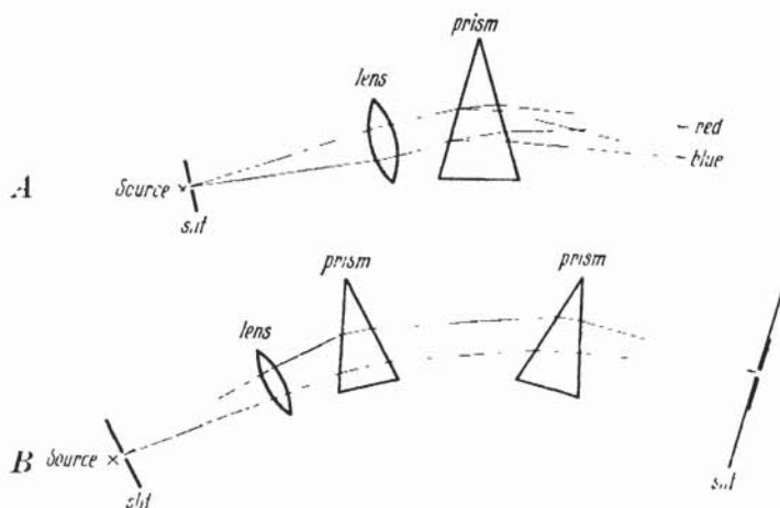
Figure 15. Spectrometers
