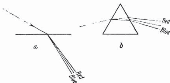
Figure 2. Refraction and Dispersion.
