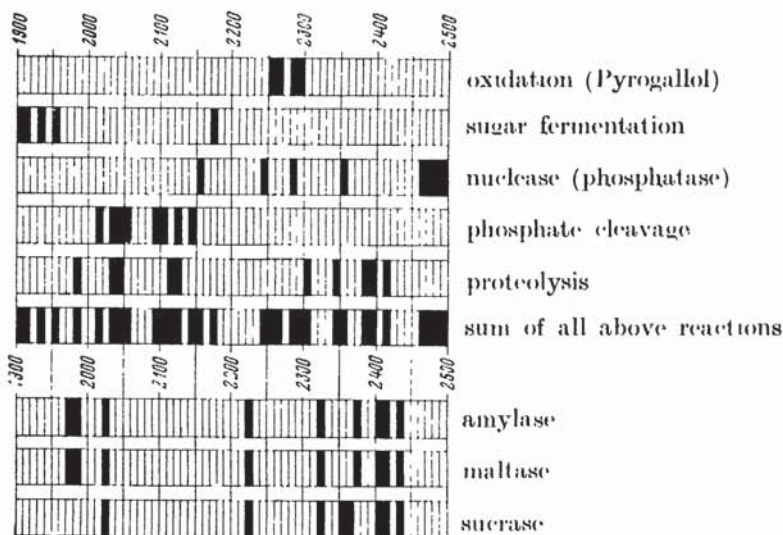
Figure 24. The spectra of some common biological reactions.
