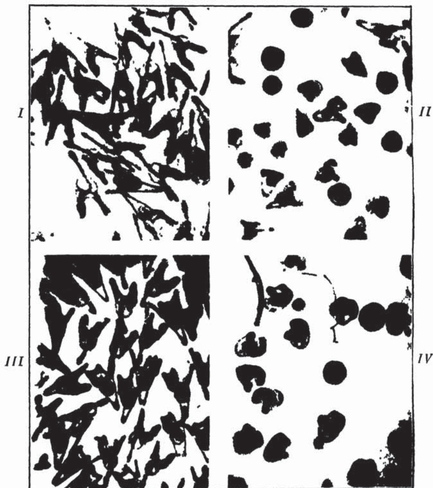
Figure 49. Larvae of the sea urchin. Paracentrotus lividus .
