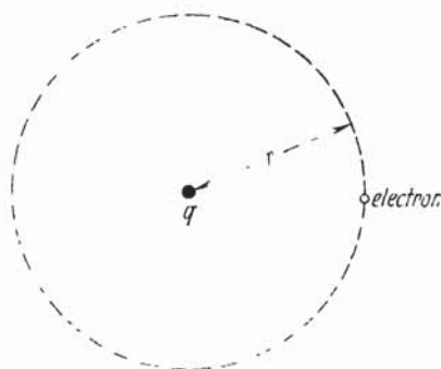
Figure 11. \rightarrow Electron in a circular orbit traveling about the positive charge q .
