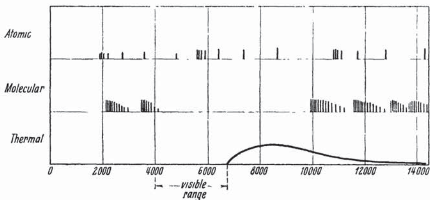
Figure 14. Representation of atomic, molecular, and thermal radiation.
