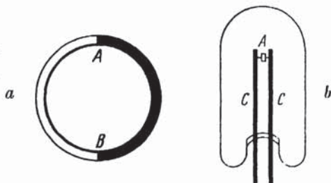
Figure 16. Thermocouples left: a two-metal thermo- element; right: a modern high- sensitivity thermocouple.
