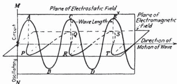
Figure 6. Diagram of an electromagnetic wave.
