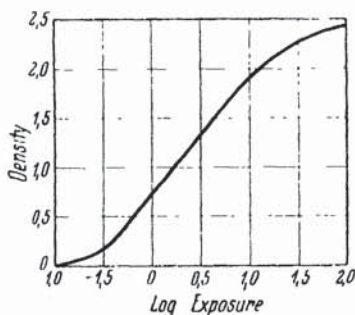
Figure 18. Characteristic curve of a photographic plate.
