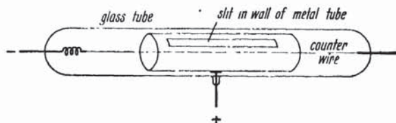
Figure 20. Photoelectric tube counter.
