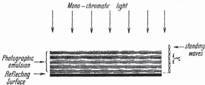
Figure 8. Experiment showing the wave nature of light.
