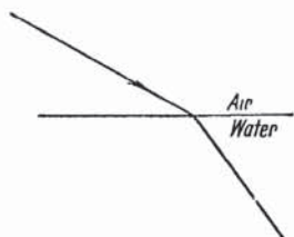
Figure 1. Refraction.
