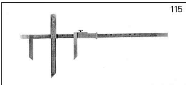
Calipers with coordinates. Scale: 20-220 mm. Weight: 0.160 kg.
