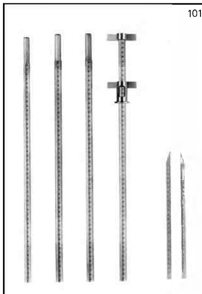
Anthropometer. Scale: 0-2100mm (0-960mm) for determination of all vertical lengths on the body. Weight: 1.450 kg.
