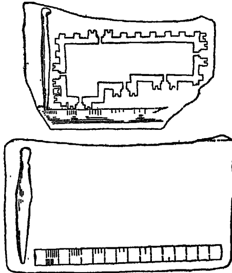
FIG. 69.—Plan of the great Temple engraved on statue of Gudēa, showing ground-plan above, and Architect's measured Rule and Stylus below. (After Déc. , pl. 15, 1, 2.)
