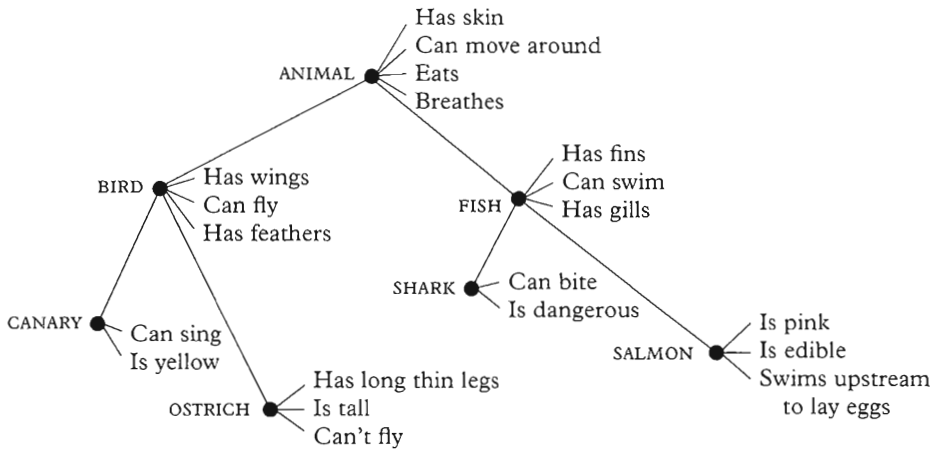
Figure 2.1 Conceptual networks
