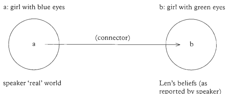
Figure 11.12 World–mind connector
