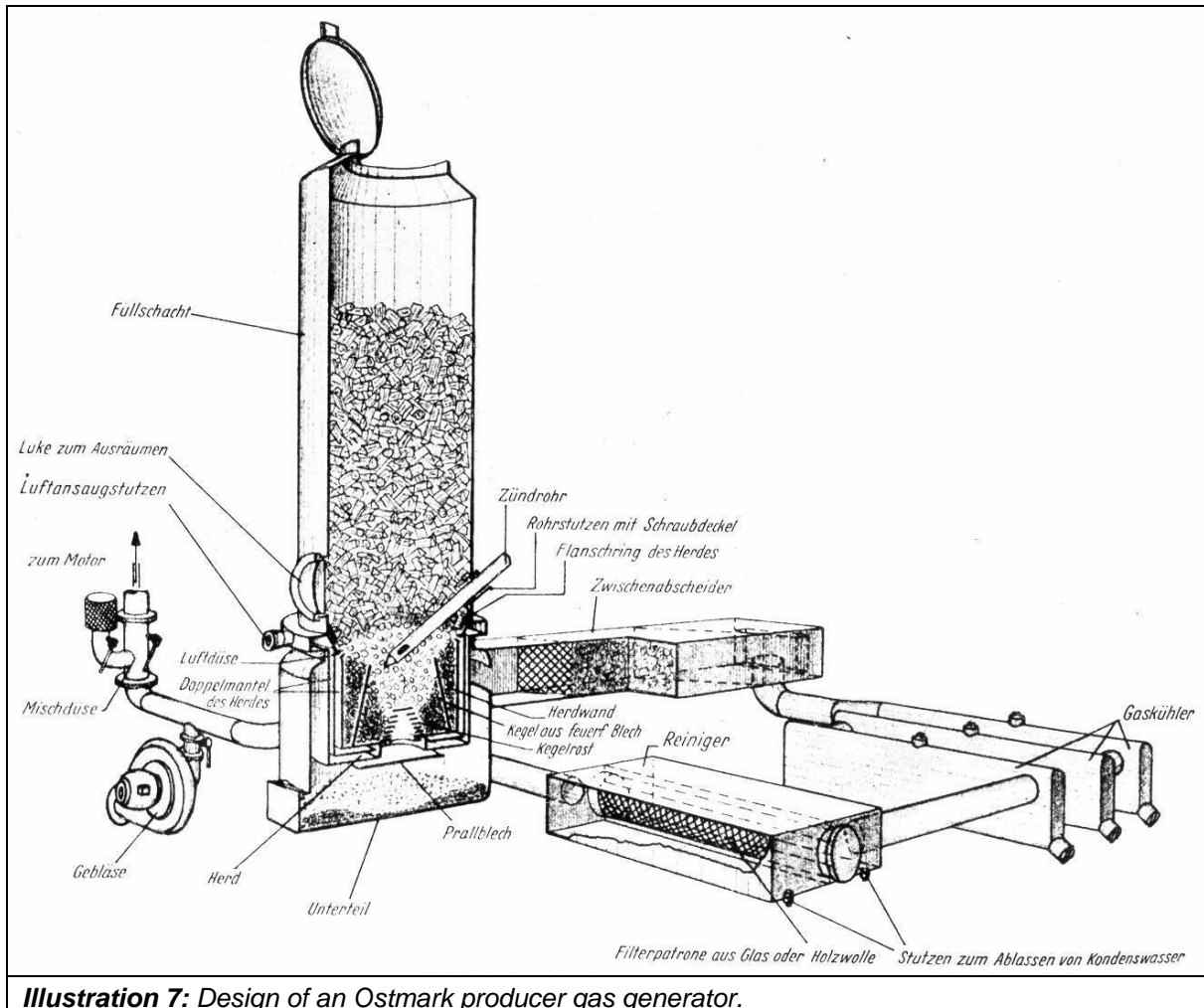
Illustration 7: Design of an Ostmark producer gas generator.
