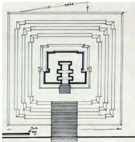
Tikal Temple II: Overhead
