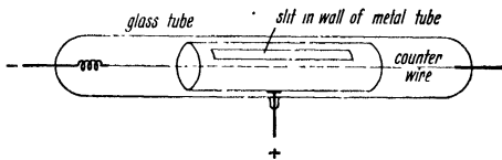
Figure 20. Photoelectric tube counter.
