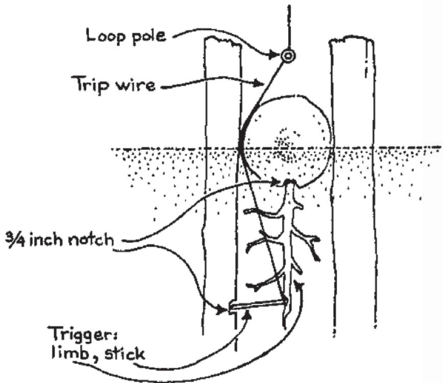
TWO POSSIBLE TRIGGER MECHANISMS
