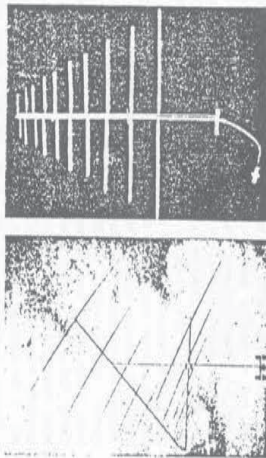
FIG. 5—Transist AB satellite antenna (left) designed by Collins Radio Company to cover 6.5 to 60 Mc; and log-periodic dipole array (right)
