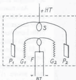
Fig. 7 -- Double triode multiple lamp with symmetrical connections and a single filament, according to the original drawing of the author's patent.
