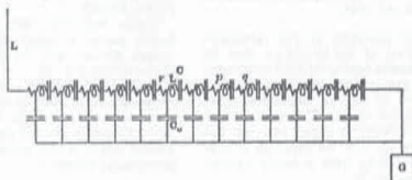
Fig. 91. Equivalent circuit of a multi-gap lightning arrester.
