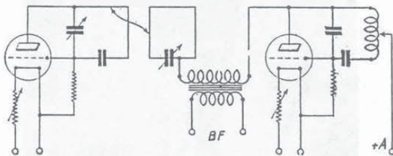
Fig. 14 -- Simplified diagram of Dr. Esau's very short wave receiver.
