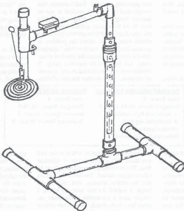
SPIRAL COIL MULTIPLE WAVE OSCILLATOR
