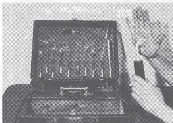
1920's era Violet Ray Massager. This device uses a small Tesla coil to drive various gas attachments which are applied to various parts of the body. Some MWOs have bulb attachments based on this device. Made by the RenuLife Company of Detroit, Michigan.
