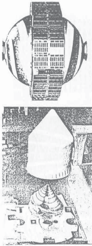
FIG. 4—First production of Dynatronics 500-to-1,000-Mc dual conical spiral antenna feed for 40-foot diameter parabolic reflector (left); Transist AB satellite antenna feed for transmission at 51, 102, 162 and 216 Mc
