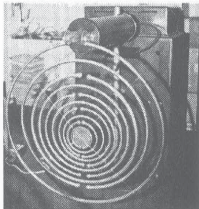
Photo showing front view of Lakhovsky Multiple Wave Oscillator antenna. The suspension in air provides for a tonal ringing.
