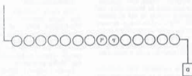
Fig. 90. Multi-gap lightning arrester.
