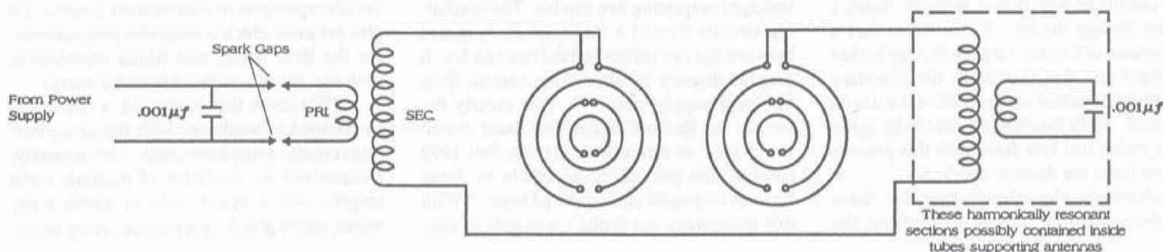
Michael Theroux's ideas for two antenna hookup based on the photographs of Lakhovsky's apparatus.
