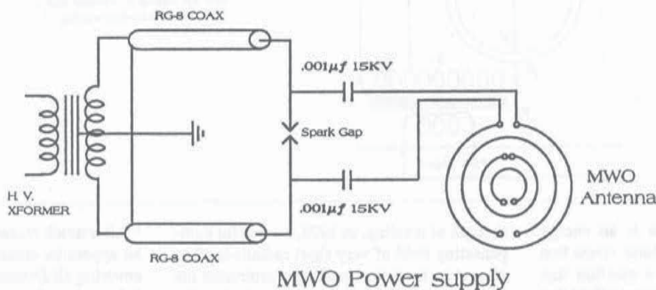
Eric Dollard's suggestions for single antenna hookup
