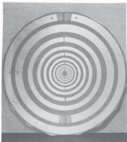
Photo 5 Yagi MWO antenna
