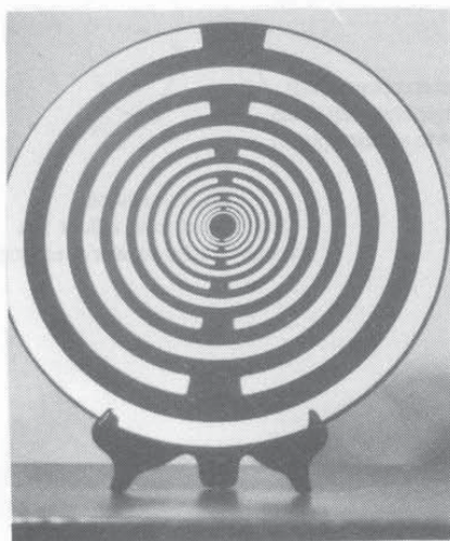
Photo 6 Golden Ratio -- Log Periodic MWO antenna
