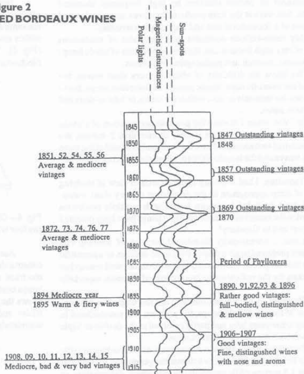
Figure 2 -- Graph showing the coincidence of outstanding vintages with the intensity of the waves emitted by the sun and corresponding to the variation in intensity: 1) of sun-spots, 2) of earth magnetic disturbances, 3) of polar lights. The graph has been established for red Bordeaux wines; the greatest intensities correspond to the outstanding vintages, the lesser intensities correspond to the years of mediocre wines. We can establish a similar graph for the other vintages, notably Bourgogne and Beaujolais wines.
