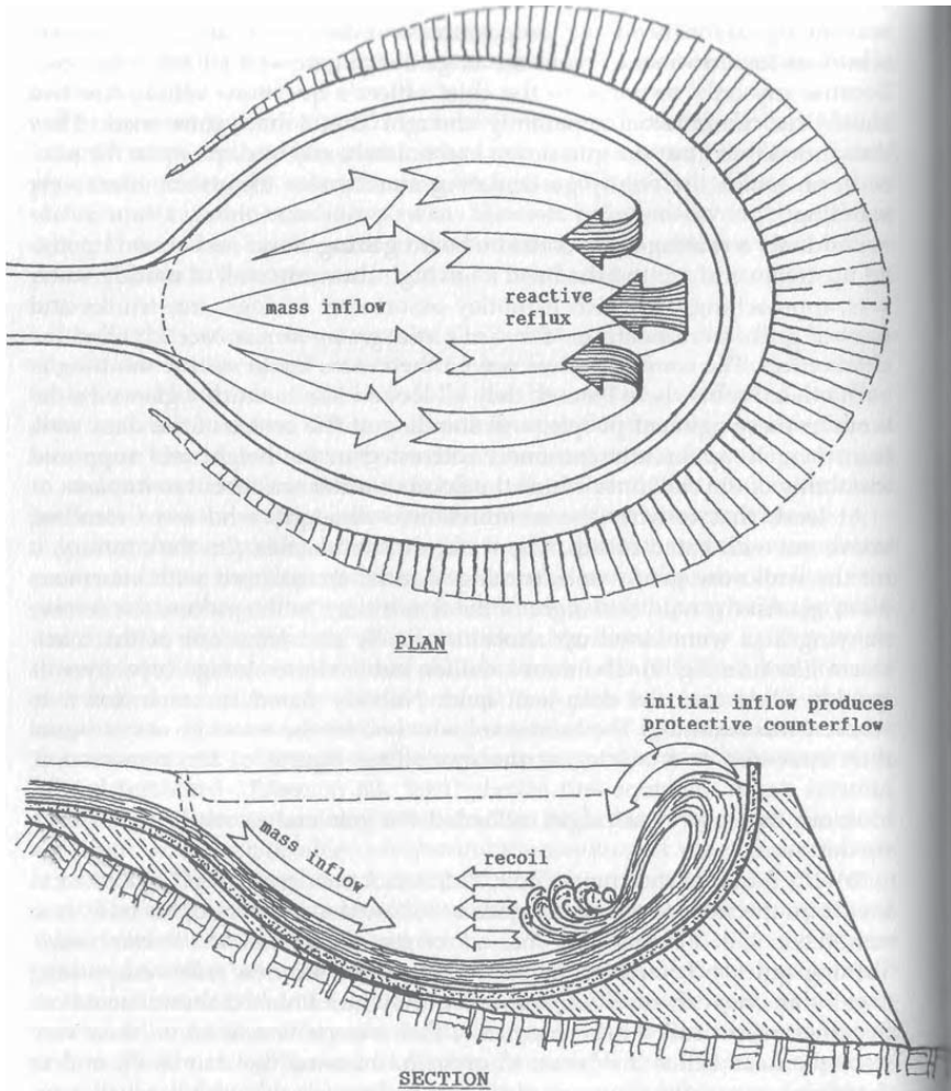
Fig. 2: The dynamics of the egg-shaped holding basin. 34
