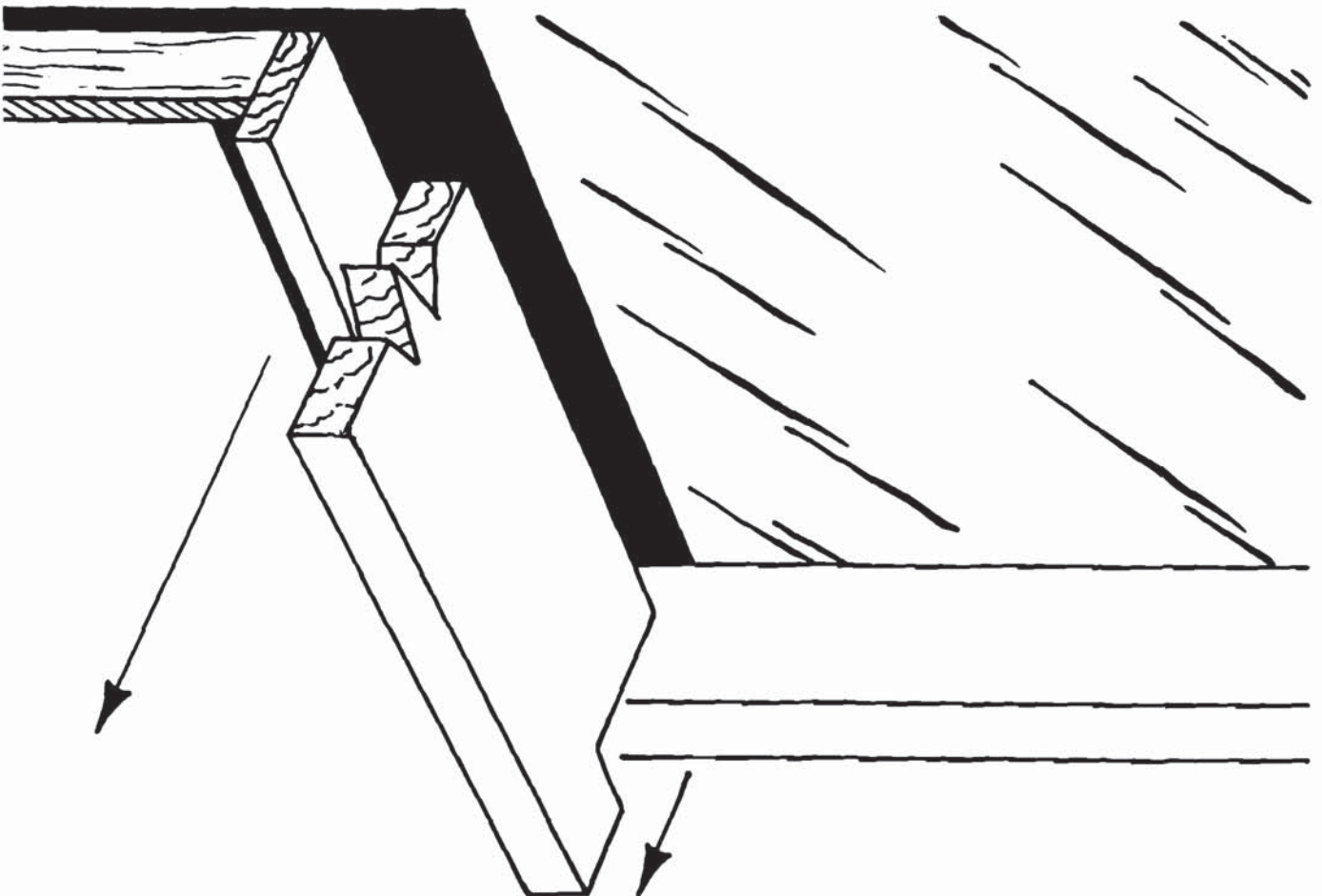
Figure 28. Removable Windowsill
