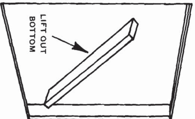
Figure 14. Opening For Countersunk Medicine Chest
