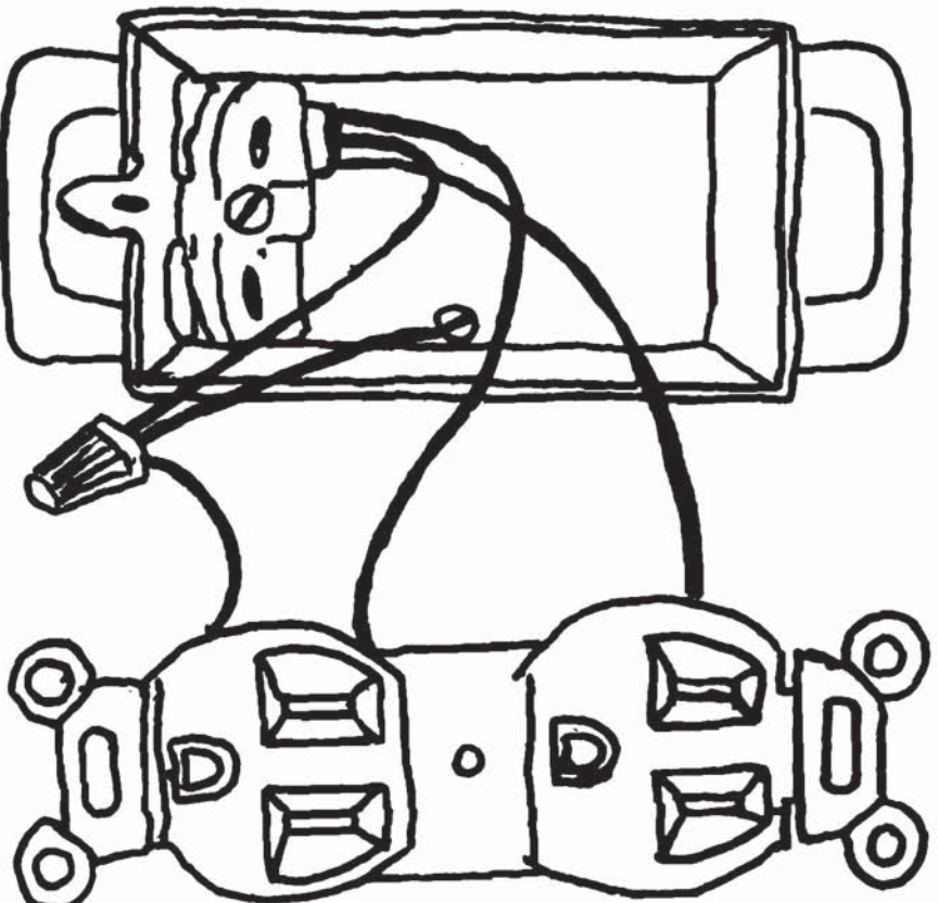
Figure 6. Wall Socket and Junction Box
