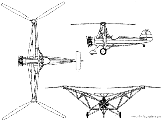
The Focke-Wulf Fw 61
