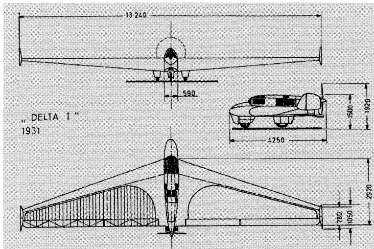
The 1931 Delta I design.
