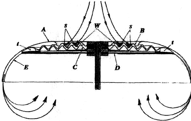
Schauberger Repulsine
