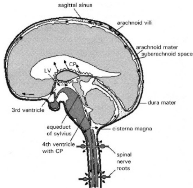
Fig. 1: Schematic illustration of the brain with the flows of cerebrospinal fluid indicated by the black arrows. The checkered area (choroid plexus) shown with the arrows pointing upwards in the inner part represents the network of blood vessels, in which the inner cerebrospinal fluid is formed. This flows out via the two ventricles shown bottom left and right. The inner grey surfaces should be imagined as permeated through and through by the plexus of nerves, which is then linked via the nerve tracts to the sense organs. (Source: A. Husemann, Der hörende Mensch und die Wirklichkeit der Musik [Human Hearing and the Reality of Music, translated and published in English by Rudolf Steiner Press], p. 74.)
