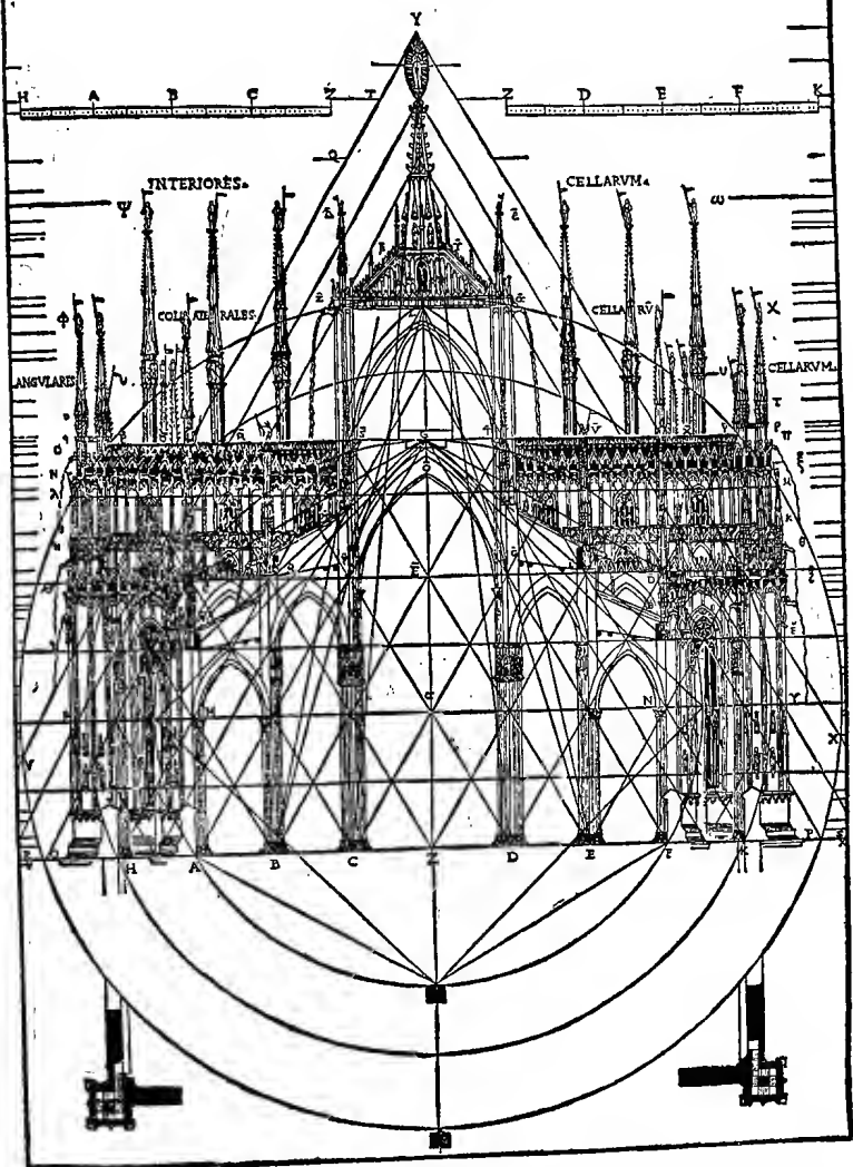
FIG. 15.—SECTION OF MILAN CATHEDRAL, FROM THE CUT IN CESARIANO'S EDITION OF "VITRUVIUS," FOLIO XV, VERSO.
