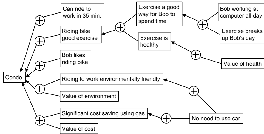
Fig. 2. Carneades [3] Argument Map of Arguments Supporting the Condo Choice
