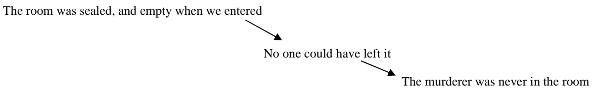
Figure 8. Beardsley's serial diagrammatic analysis
