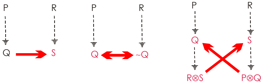
Figure 22. Pollock diagrams
