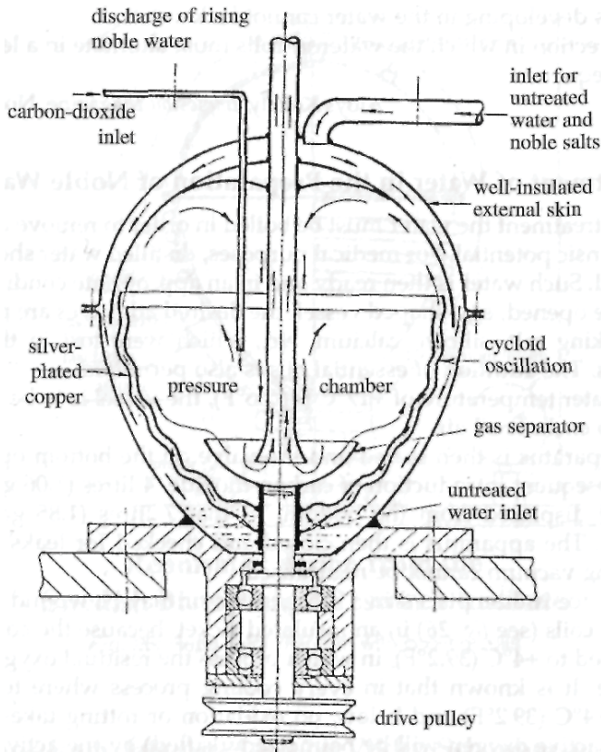
Fig. 25: Repulsator cross-sectional drawing
