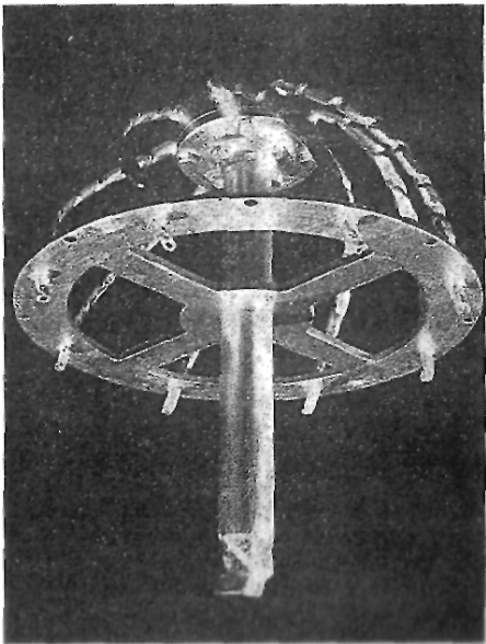
Fig. 13: Bioturbine rotor with whorl-pipes
