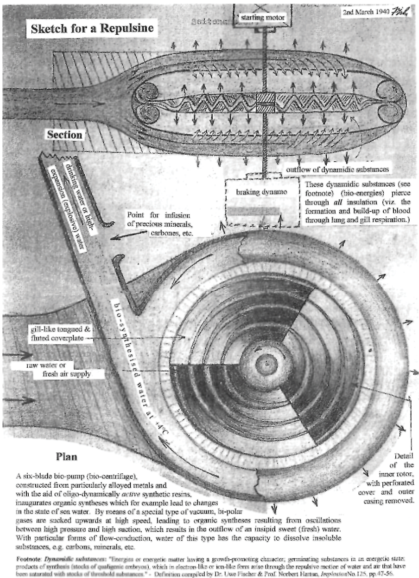
Fig. 32: Repulsine patent double membrane
