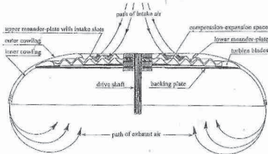
(e) Section through the machine.
