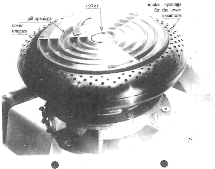
Fig. 31: Repulsine patent
