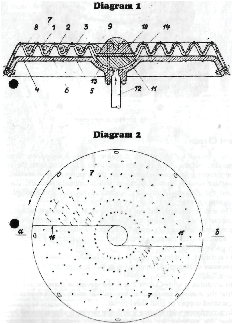
Fig. 30: Repulsine patent No. 146 141
