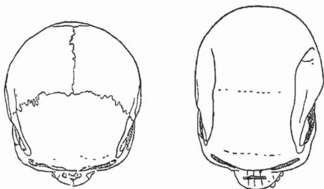
SHORT SKULL (brachycephalous) LONG SKULL (dolichocephalous) (After de Mortillet)
