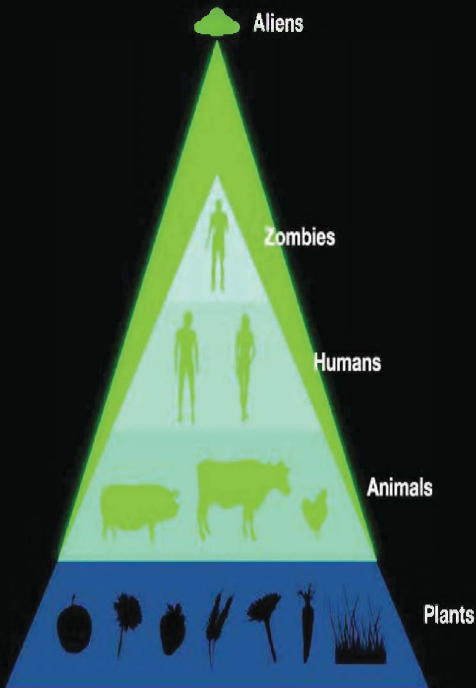
The food chain.
