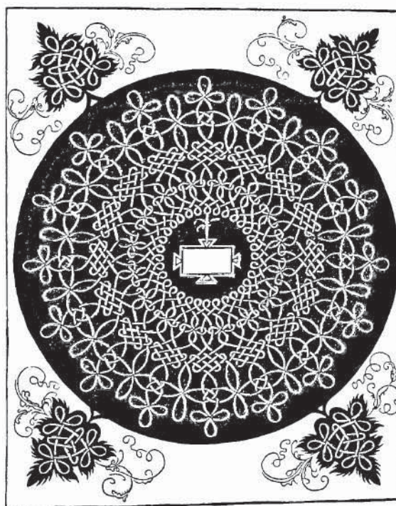
Figure 23 One of Durer's 'Sechs Knoten'
