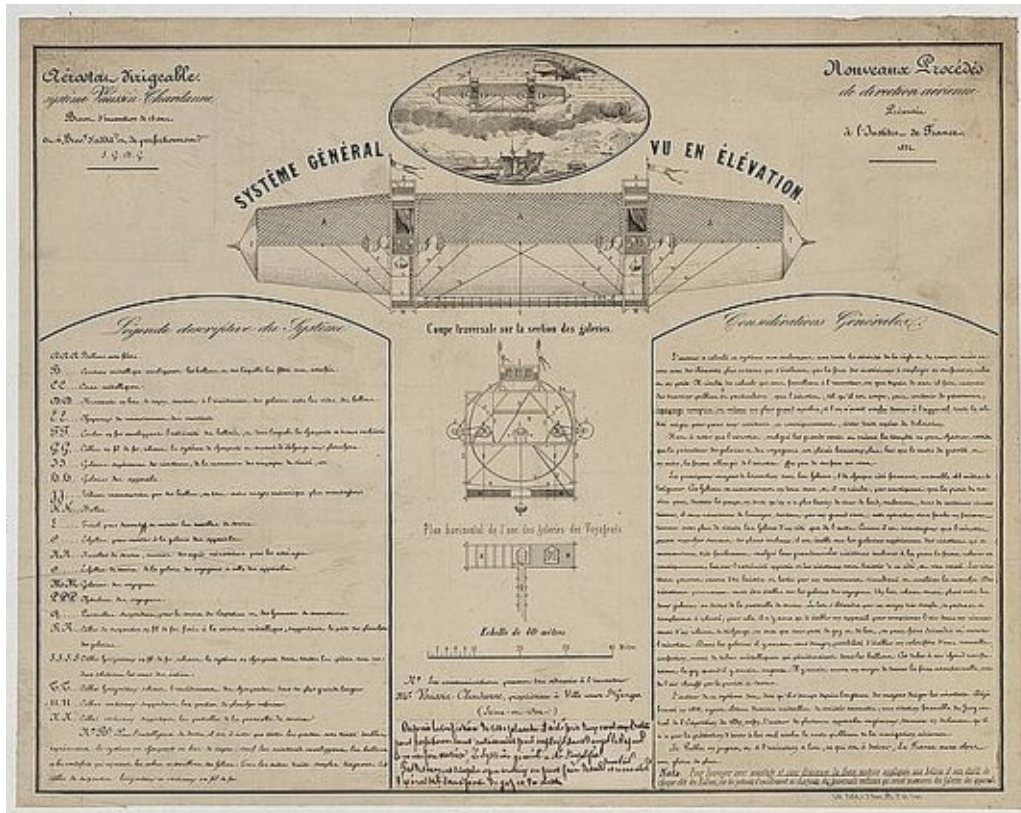
French blueprints/patent of an airship design, 1852.
