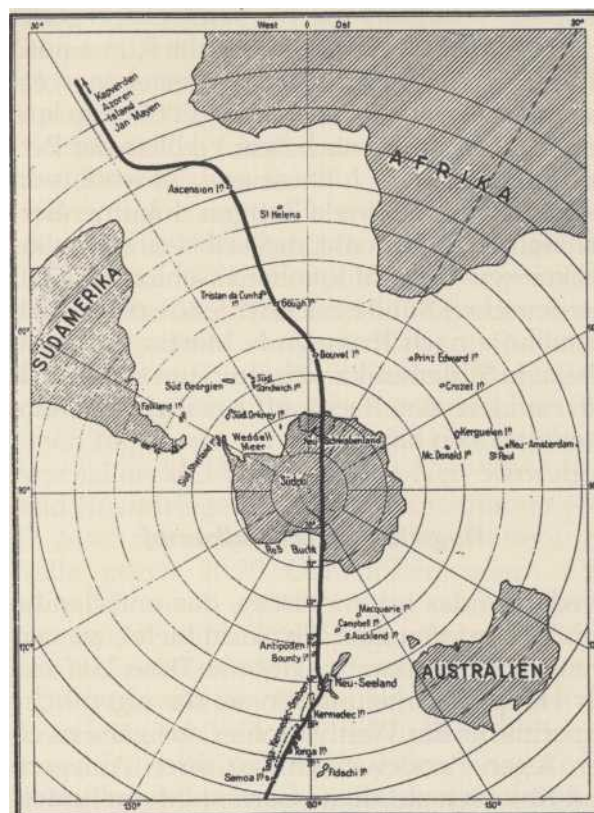
Example from the Internet: Alleged underwater warm water trench under the Antarctic continent that can be used as a submarine route.
