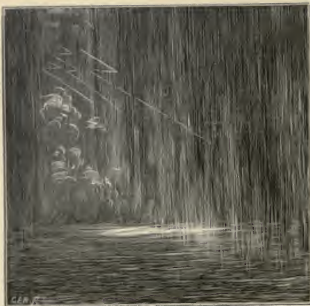
THE PRIMEVAL STORM.
