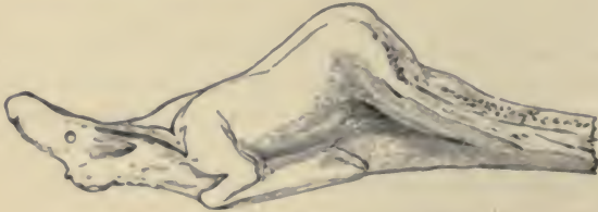
A SPECIMEN OF PRE-GLACIAL CARVING.
