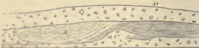
STRATIFIED BEDS IN TILL, LEITHEN WATER, PEEBLES SHIRE, SCOTLAND.
