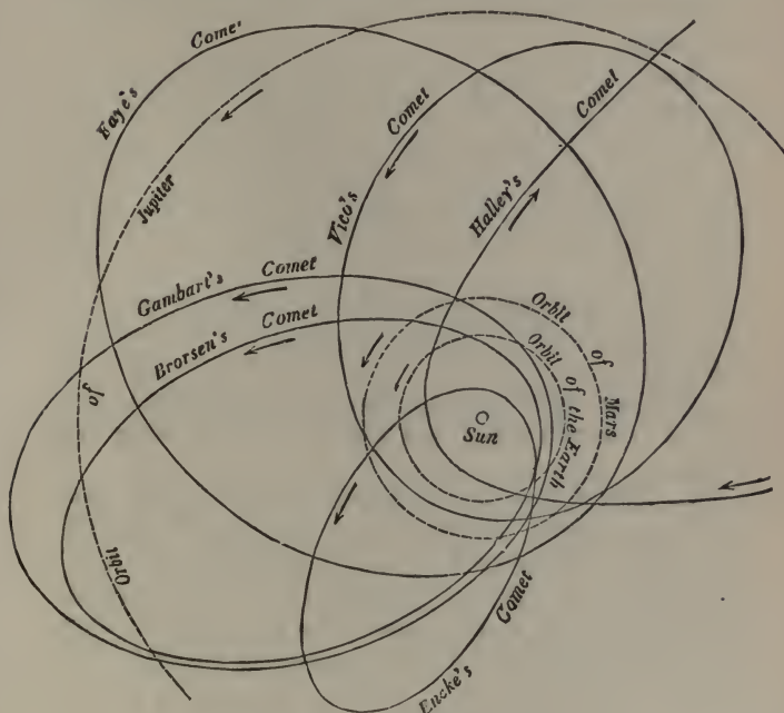
ORBITS OF THE PERIODIC COMETS.
