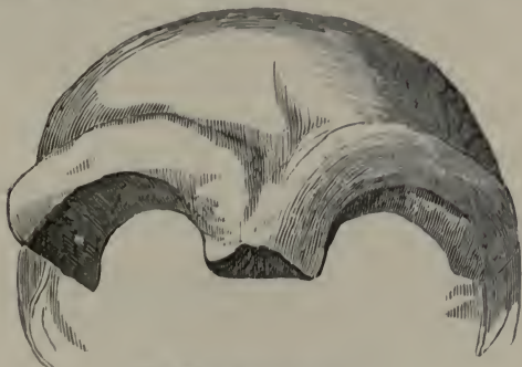
THE NEANDERTHAL SKULL.
