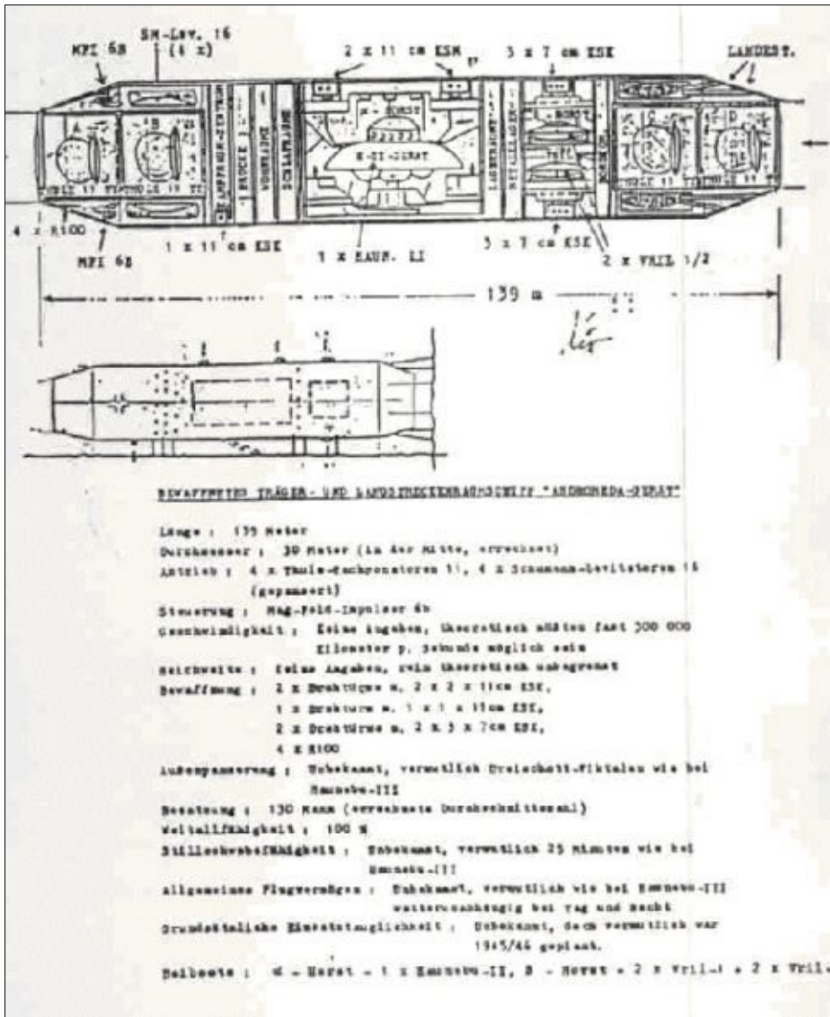
Arthur Sack's circular flying machine prototype, phase 2.
