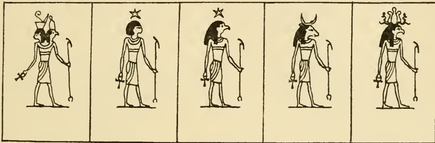
Venus. Mercury. Mars. Saturn. Jupiter.
