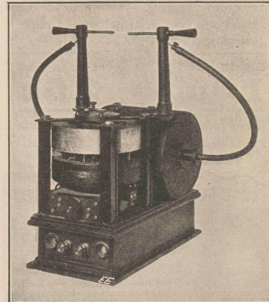
Fig. 18. Tesla Transformer With Mercury Jet Interrupter.
