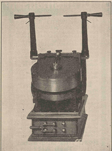
Fig. 17. Tesla Transformer With Adjustable Mercury Controller.
